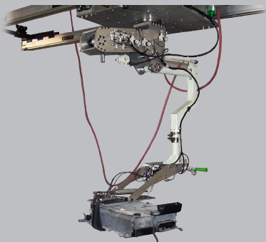
Custom Hybrid Battery Installation Manipulator
